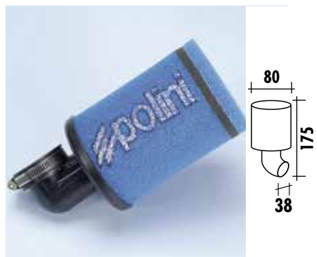
203.0029 | Ø38 - Scooters Evolution PHBG
