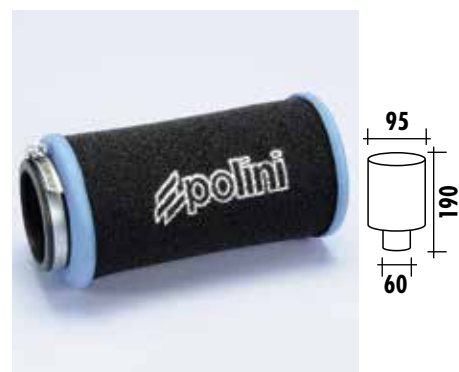
203.0164 | Ø60 - Scooters - Carburetor POLINI CP
